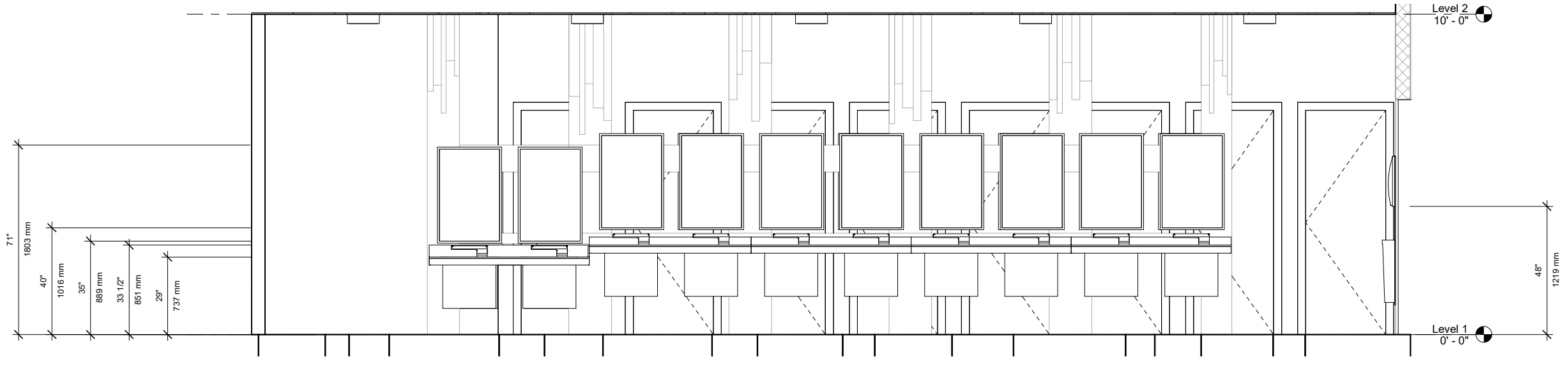
④ ADA Sink Bank Section View 1/2" = 1'-0"
