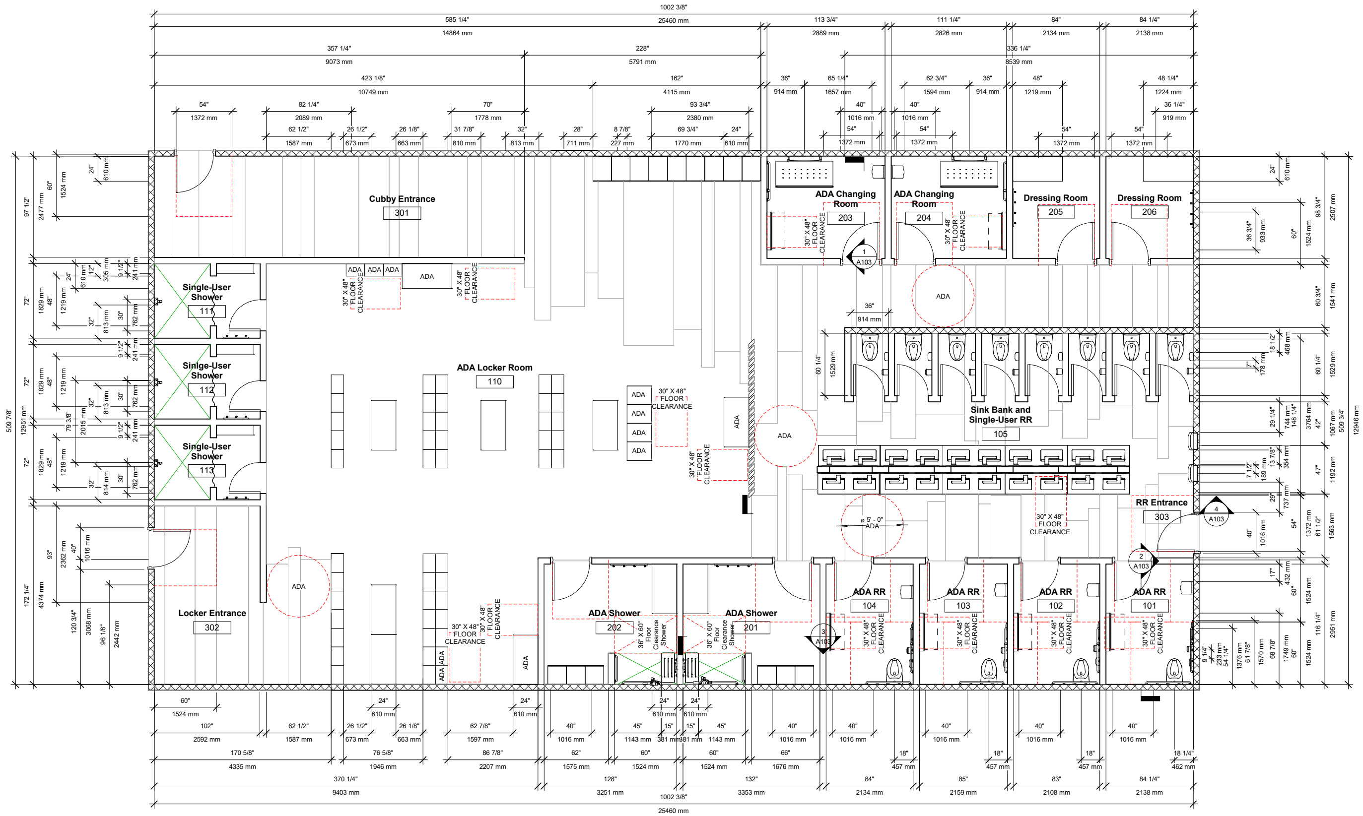
① Dimension Plan 1/4" = 1'-0"
