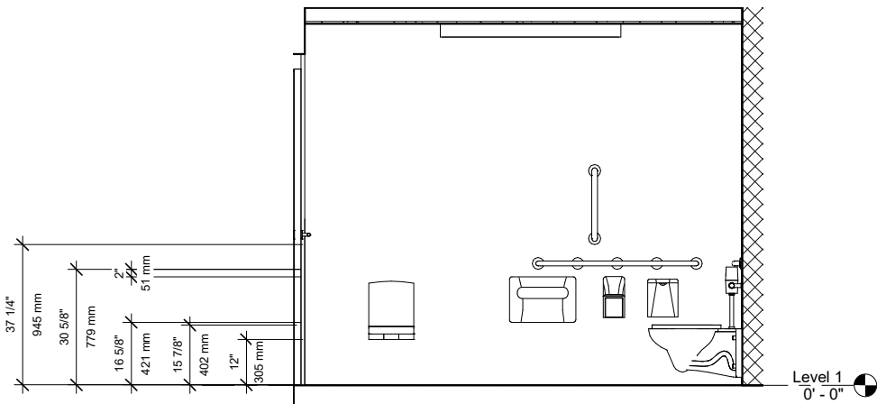
② ADA Restroom Accessories Heights 1/2" = 1'-0"
