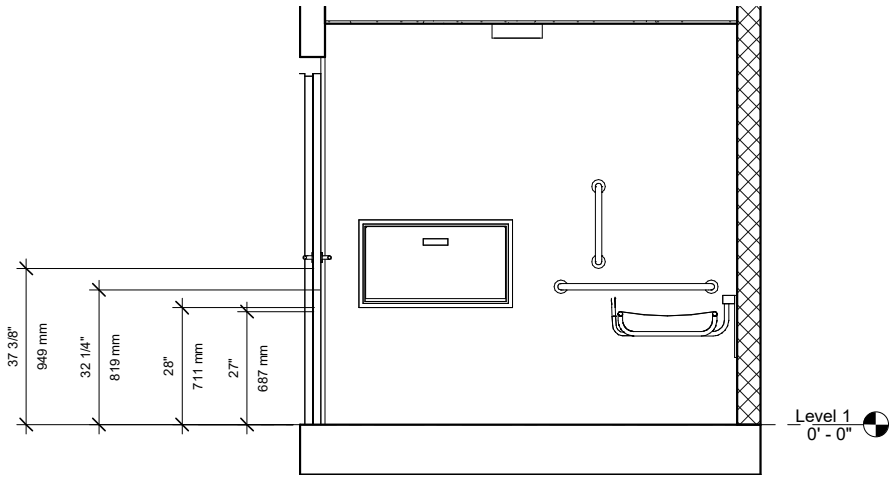
① ADA Changing Room Section View 1/2" = 1'-0"
