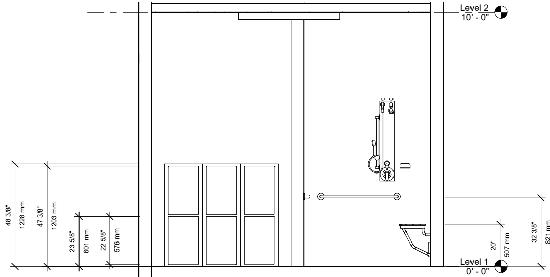
③ ADA Shower Section View 1/2" = 1'-0"
