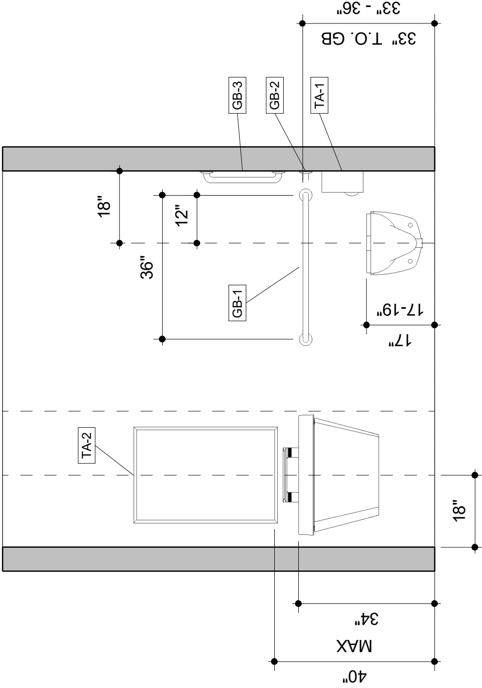
4 FRONT | ACCESSIBLE TOILET ROOM 1/2" = 1'-0"
